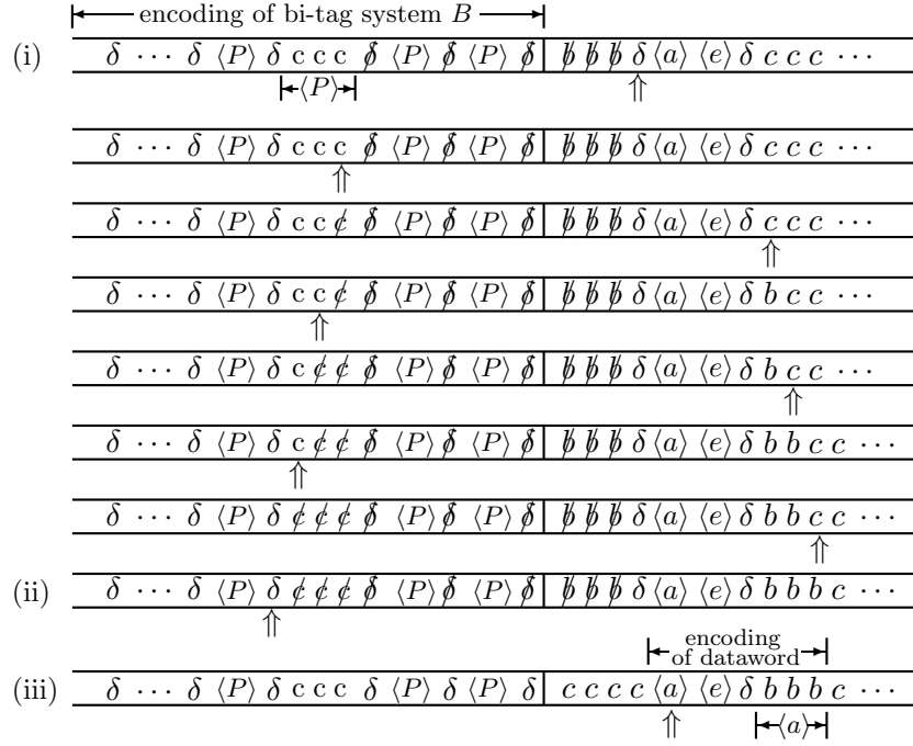
Figure 6.2.2: Printing of an encoded production during simulation of a production of B . Over a number of timesteps, the encoded production \langle P \rangle , indexed in configuration (i) of Figure 6.2.1, is printed to the right of the encoded dataword.
