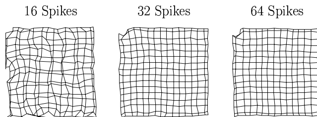
Figure 3: Final states of the topographic mappings between the neuromorphic chip's retinal array and a target sheet for three different levels of spike binning per iteration. The number of spikes per bin used to generate a map is indicated immediately above the map.
