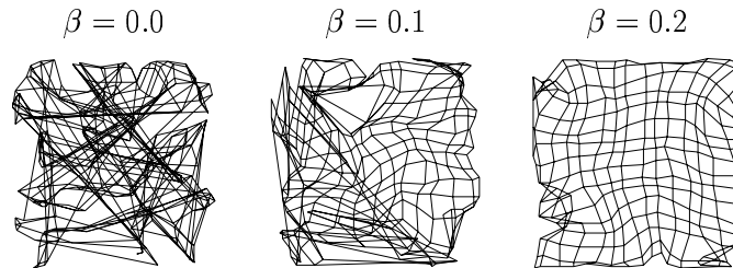
Figure 5: Final states of the topographic mappings between the neuromorphic chip's retinal array and a target sheet for three different values of the initial topographic bias parameter \beta . The value of \beta used to generate a map is indicated immediately above the map. In all cases, 32 spikes are binned per iteration.
