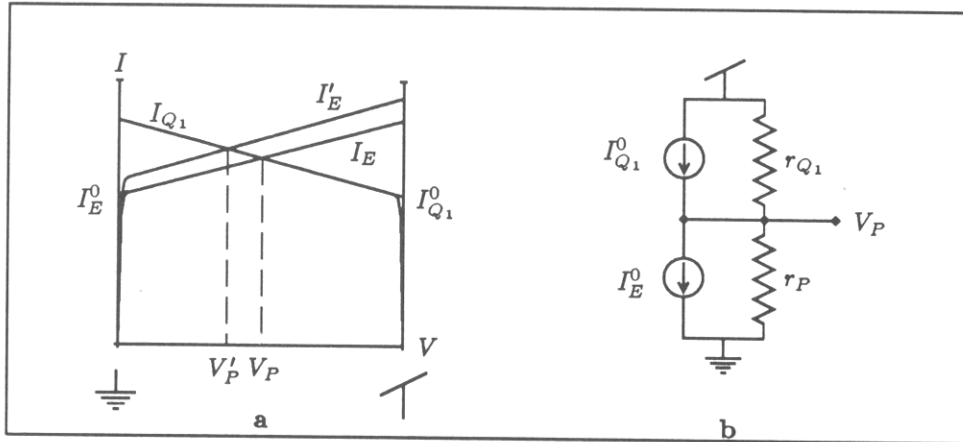
Figure 2. The first stage of amplification. a: The curves show the current through the phototransistor P and feedback transistor Q_1 as a function of the voltage V_P . Since I_P = I_{Q_1} the intersection gives the voltage V_P . b: An equivalent circuit model for these transistors in the linear region. The Early effect leads to drain/collector resistances inversely proportional to the value of the current source.
