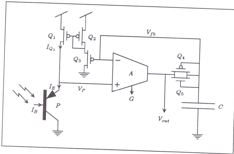
Figure 1. The photoreceptor circuit.
