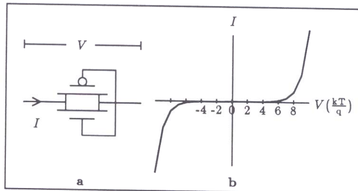
Figure 3. a: The hysteretic element. b: I - V characteristic.
